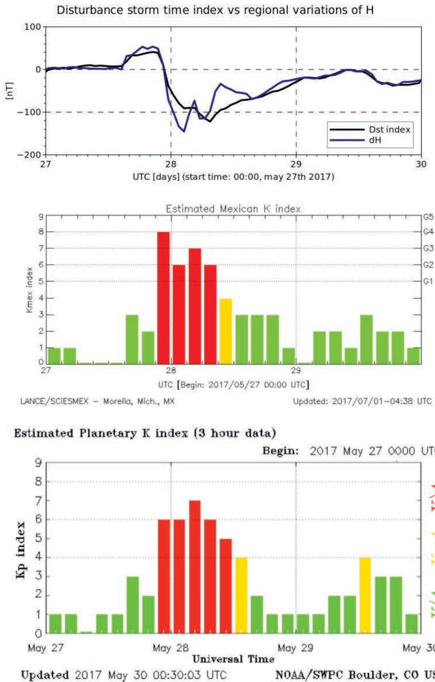
Figure 2. Upper: Dst (black) index and hourly averaged dH (blue). Middle: Estimated Kmex index. Bottom: Estimated Kp by SWPC/NOAA.
