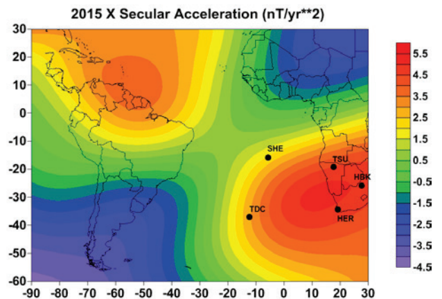
Figure 6. A map showing X-component secular acceleration at the Earth's surface for 2015.0 in the South Atlantic and southern African region as determined using the CHAOS-6 model. The positions of the different observatories used in the investigation are indicated by their respective IAGA codes and black dots.
